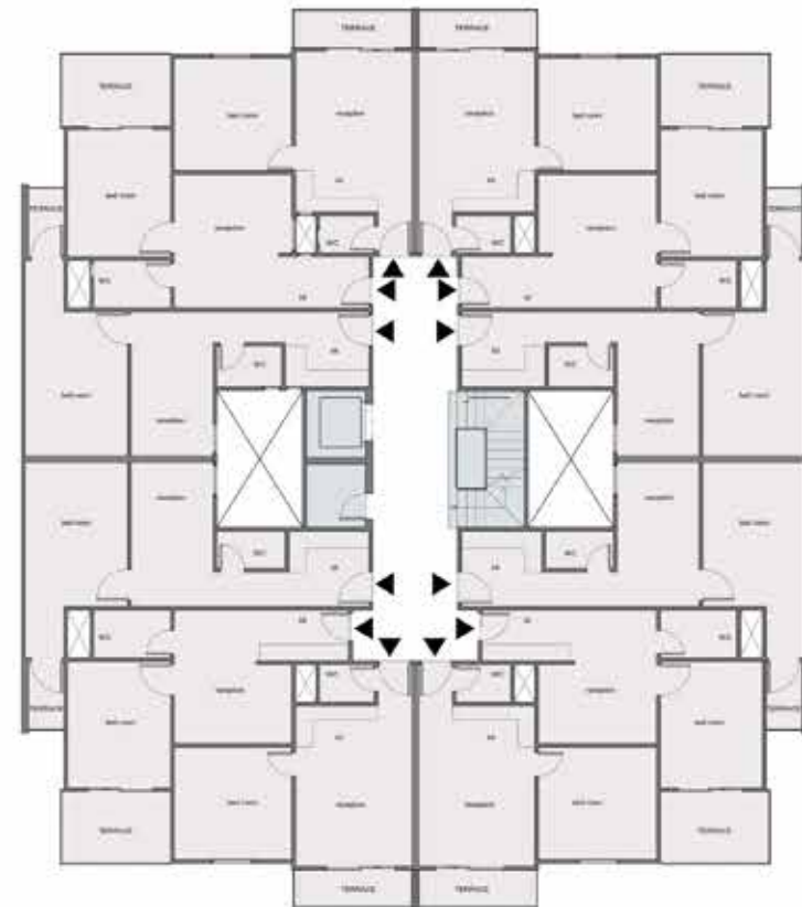
BULDING TYPE A FIRST FLOOR
