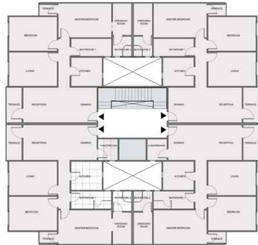
BULDING TYPE A FIRST FLOOR
